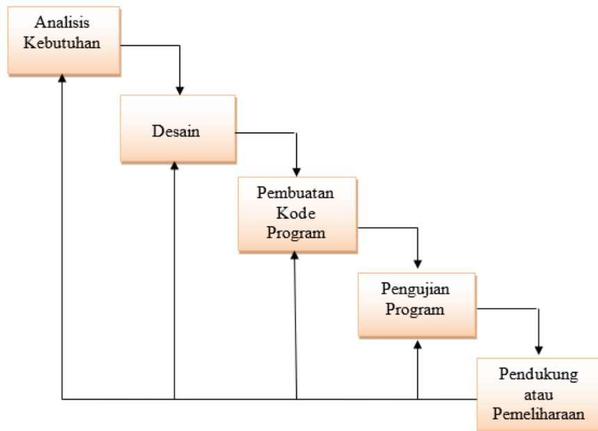
Gambar 1. Tahapan Waterfall
