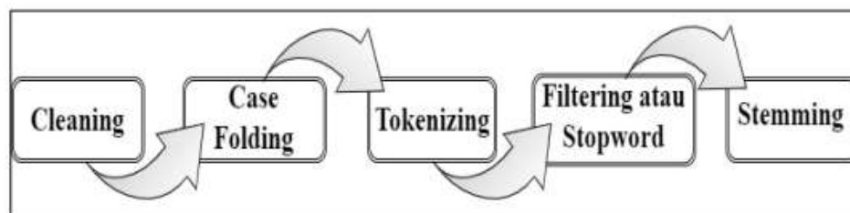
Gambar 1. Preprocessing Data
